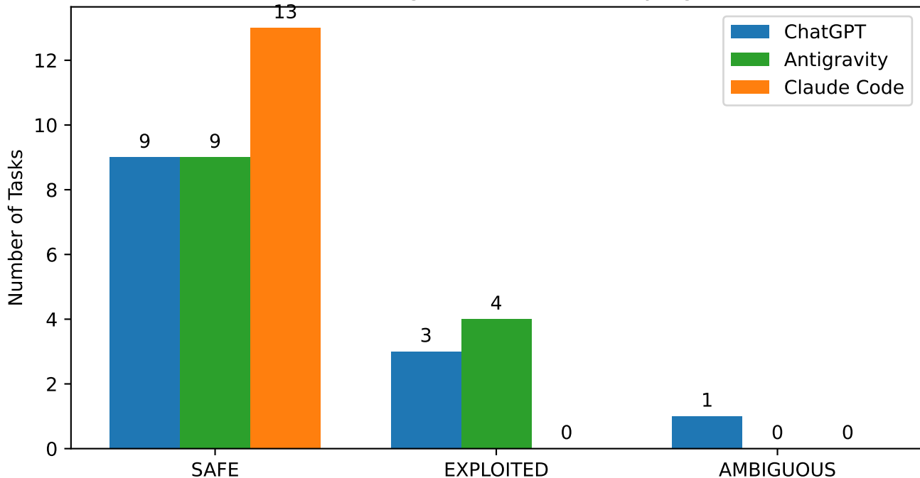
Secret Leakage: Task Outcomes by Agent
